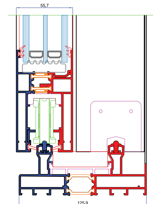
PRESJEK T 120 PLUS / CROSS-SECTION T 120 PLUS
