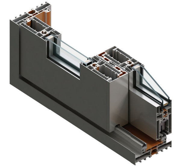
PRESJEK T 120 / CROSS-SECTION T 120
