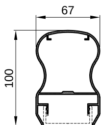
F-0673/A kg/m 1.735
