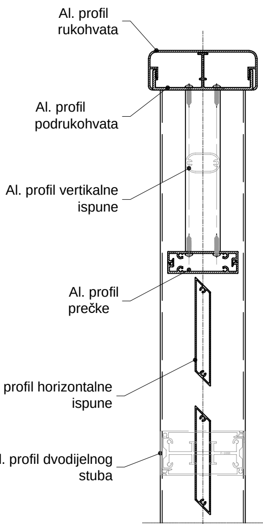
Stub 45x86
